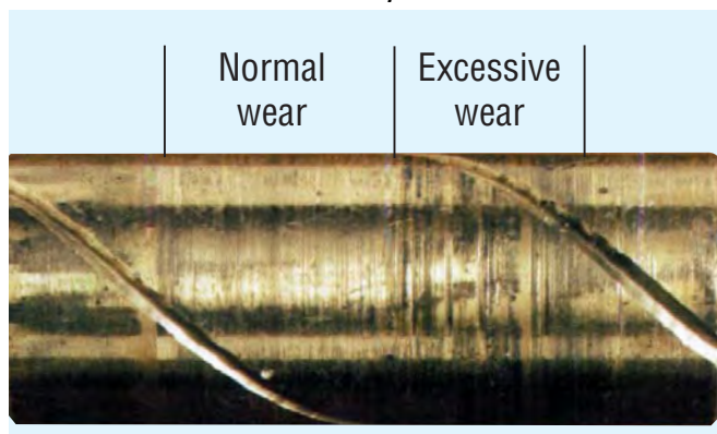
Bronze Idler Pins - Normal/Excessive Wear
